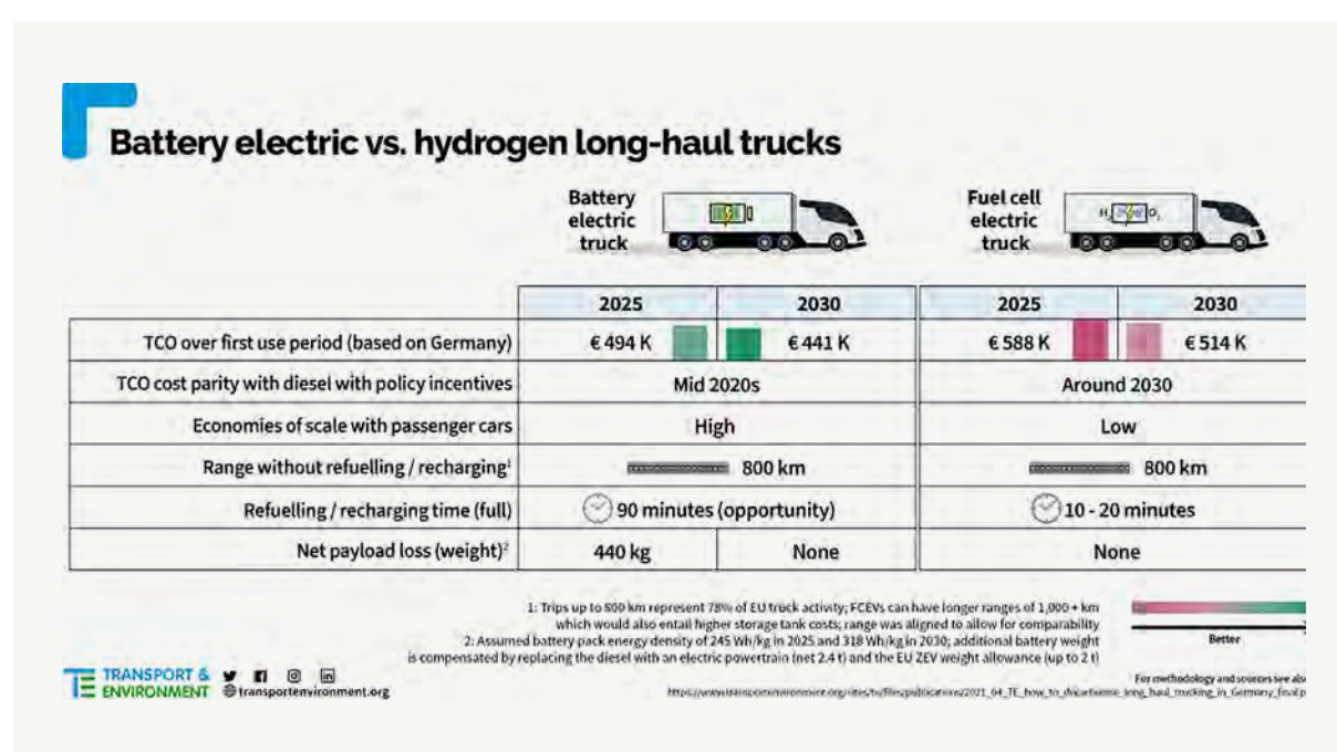
Figure 37: Battery electric v hydrogen long-haul trucks 71
