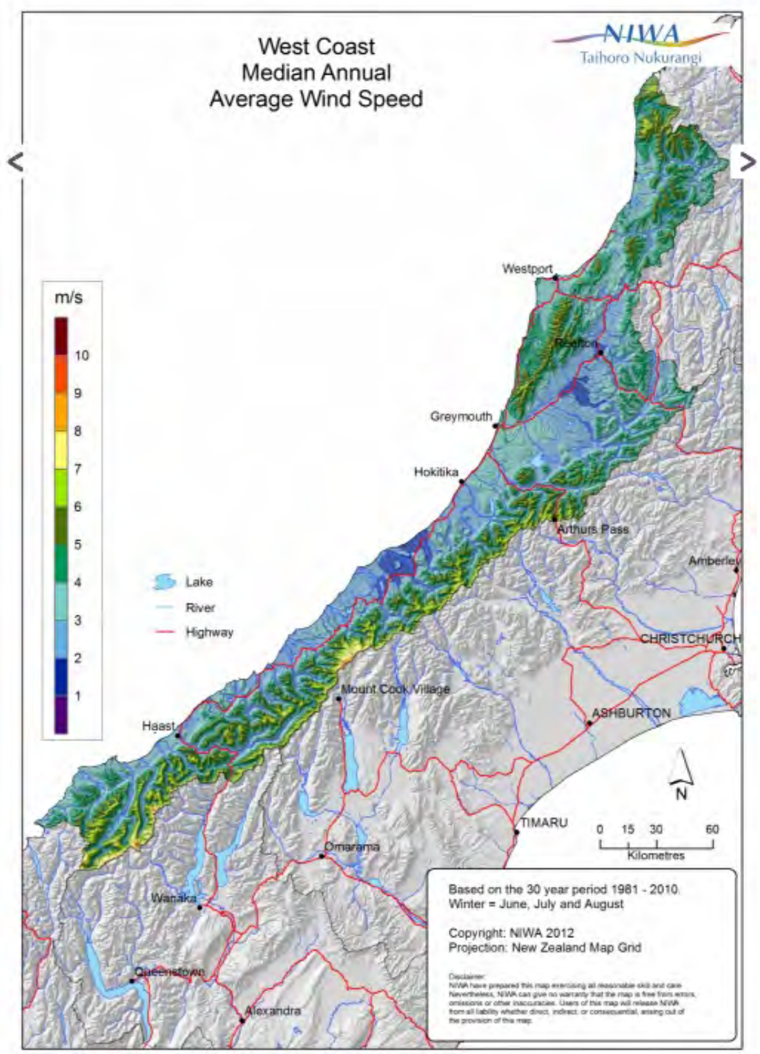
Figure 25: West Coast annual average wind speed 50
