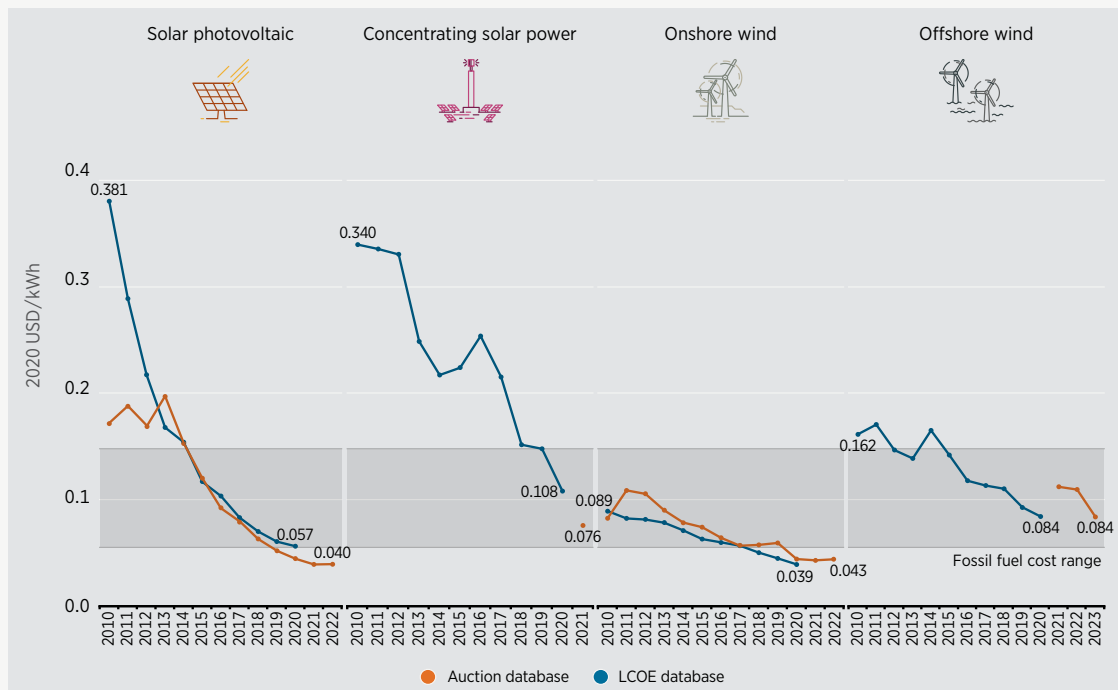
Figure 12: The global weighted-average LCOE and PPA/auction prices for solar PV, onshore wind, offshore wind and CSP, 2010-2023
