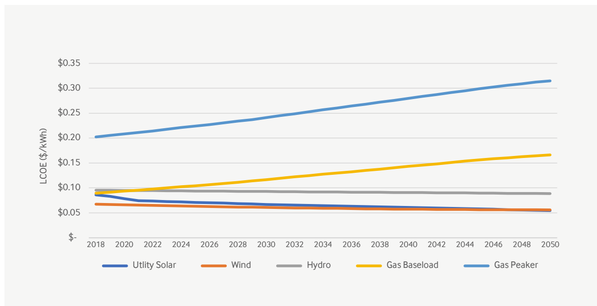
Figure 20: NZ$ cost of energy from different sources as technology and carbon prices evolve
